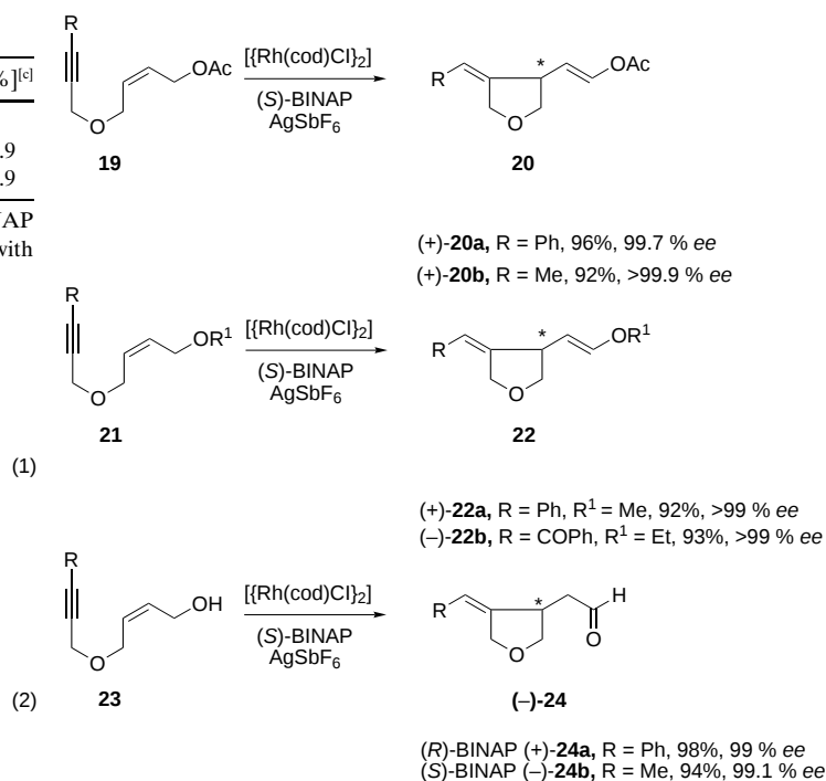
Scheme 1. Highly enantioselective Alder–ene reactions of enynes substituted at the allylic terminus.
